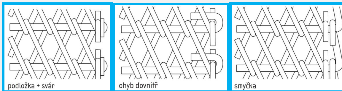
Plate + weld
